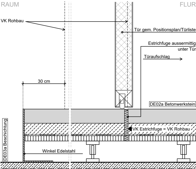
8 Anschluss Tür SDfz - DE02/DE03
