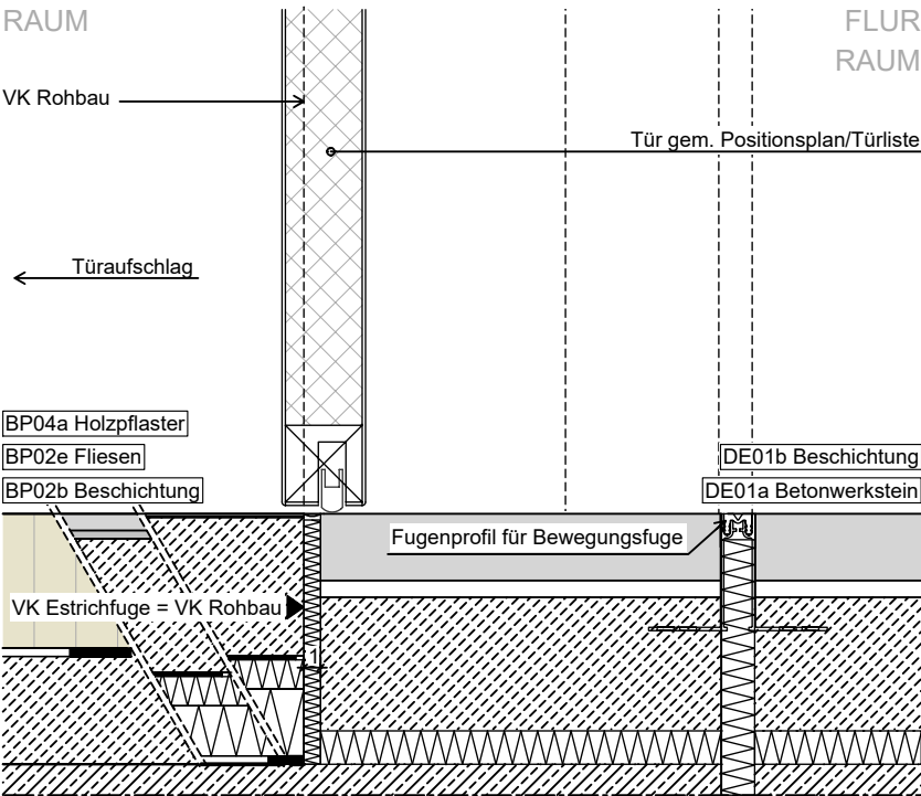
9 Anschluss Tür SDfz - DE01/BP02, BP04
