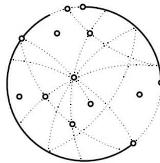
COMPLEXITY NETWORKS
