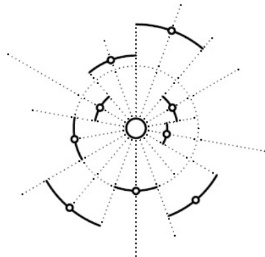
PLANETARY BOUNDARIES
