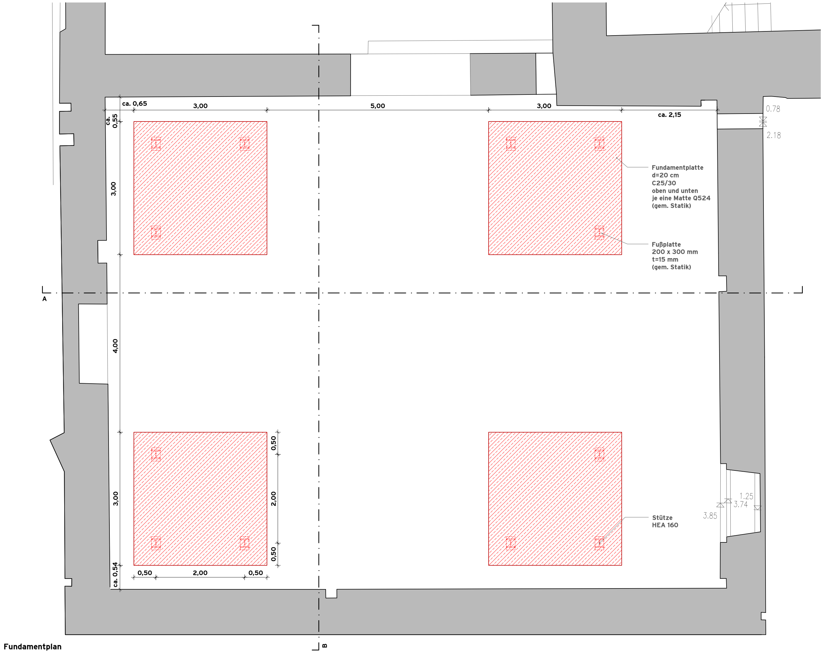
Fundamentplan
