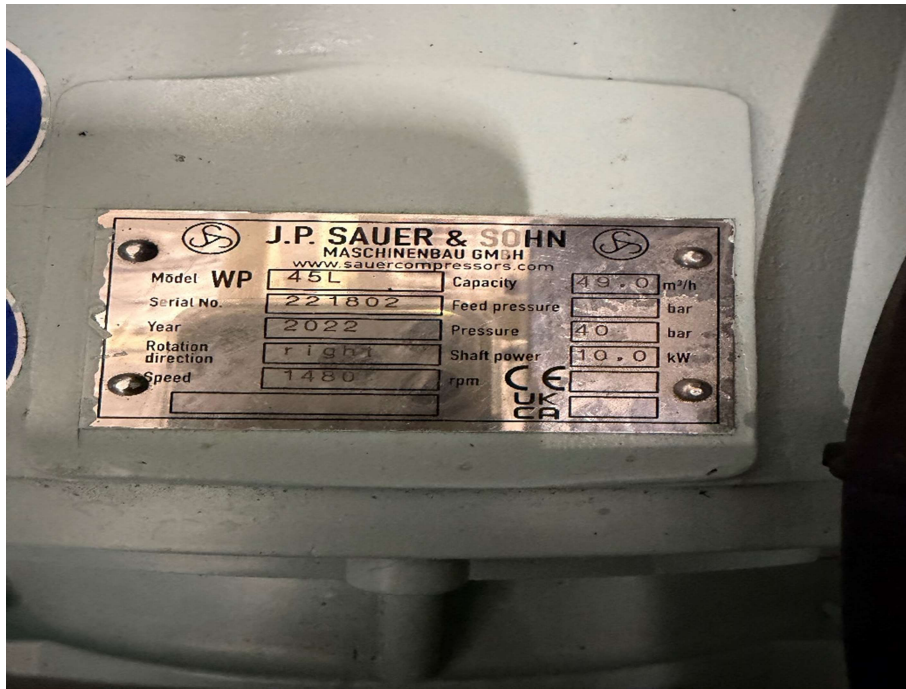
Startluftkompressor 2 (651G0002)
