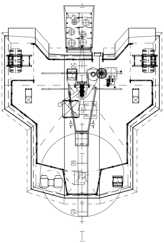
Peildeck
