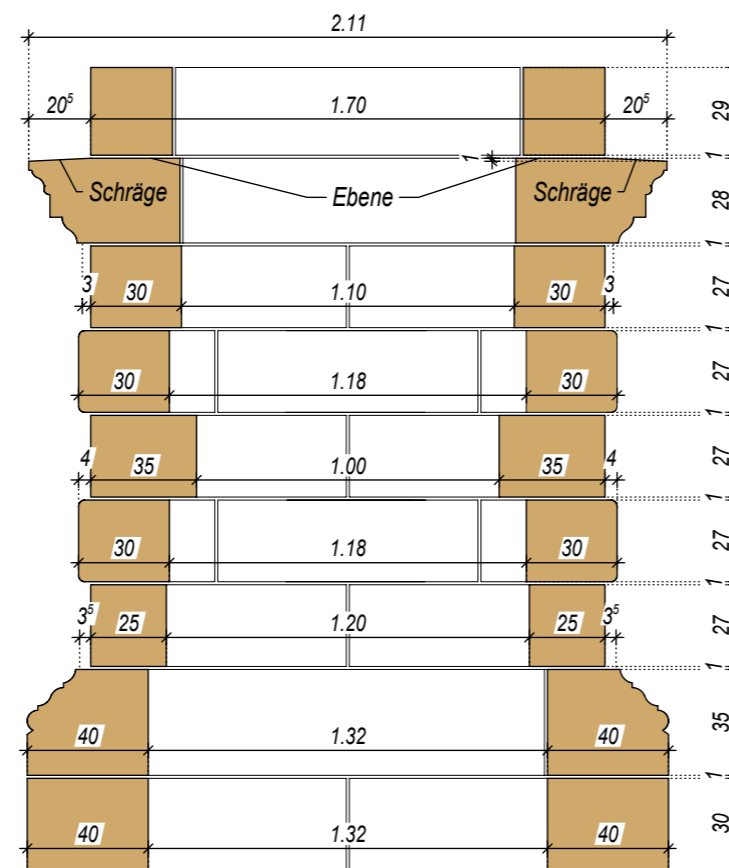
Schnitt SC1 - SC1 M = 1:25
