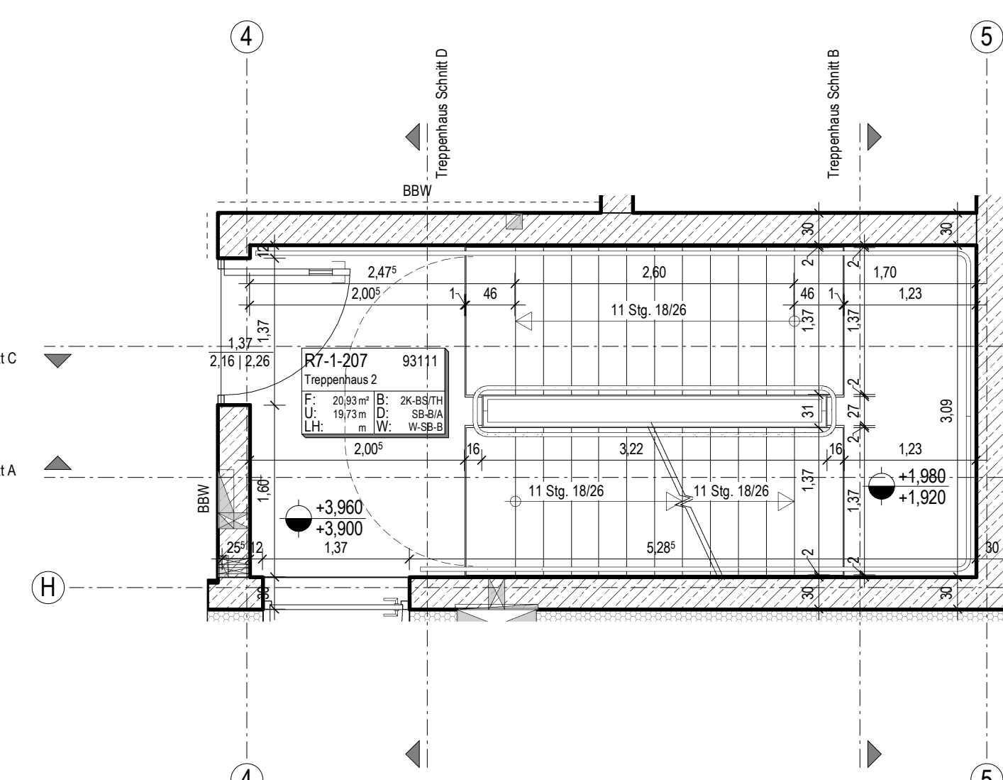
Grundriss 1OG
