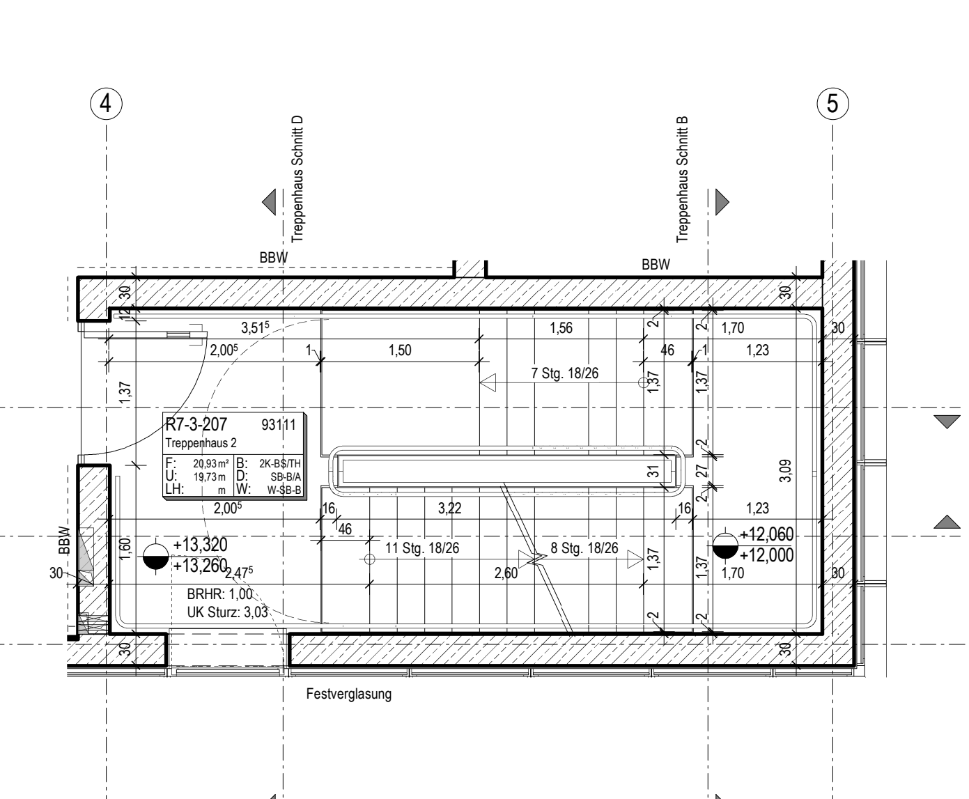
Grundriss 3OG
