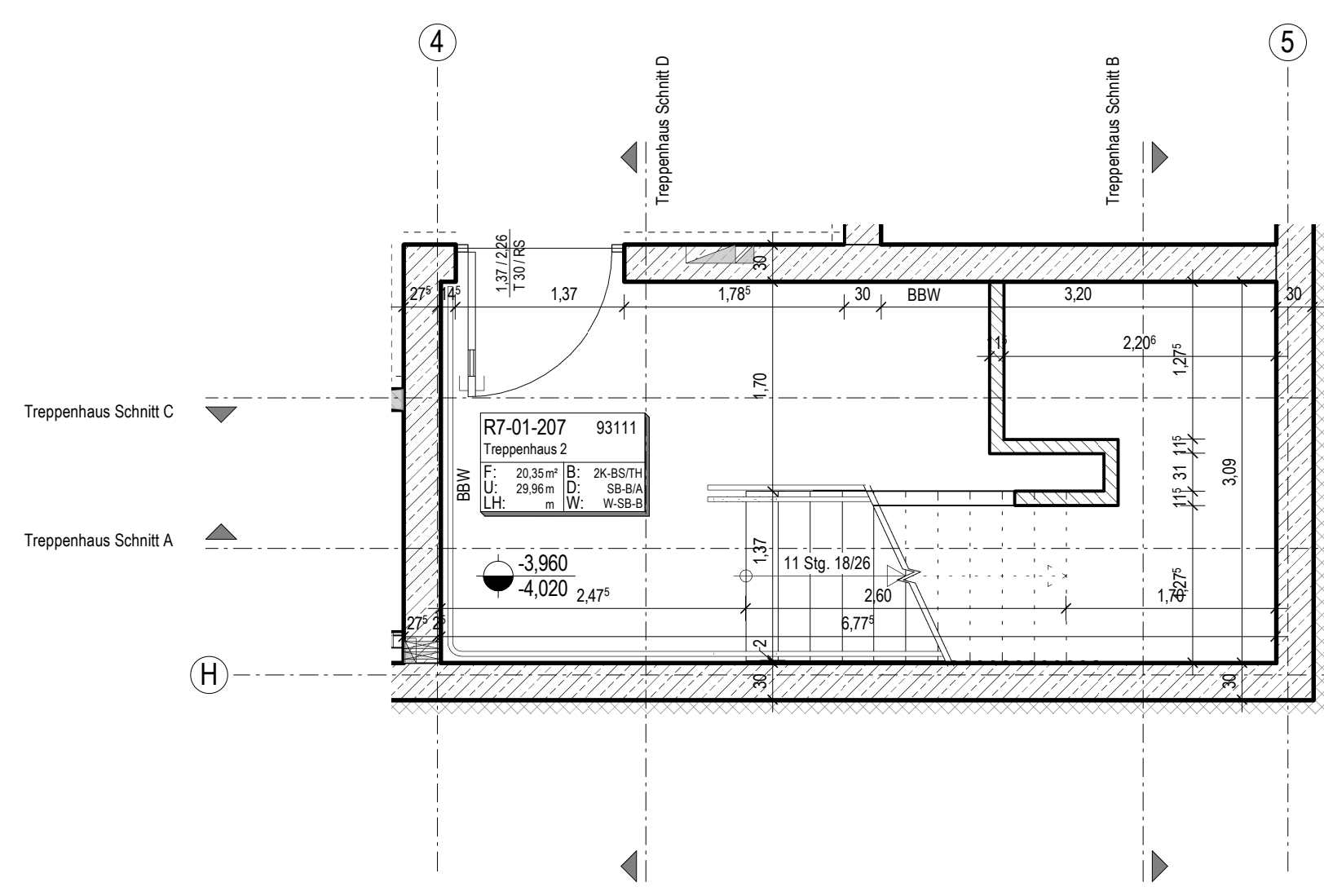
Grundriss 1UG
