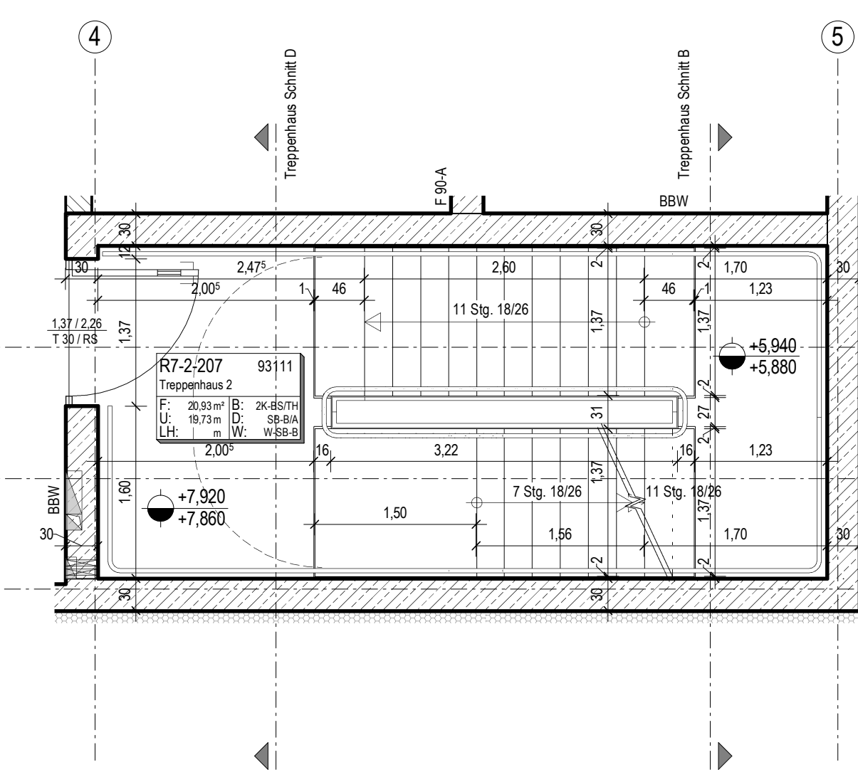
Grundriss 2OG
